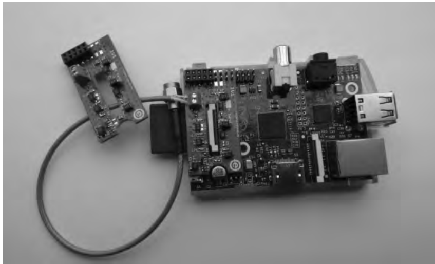
Figure 9. - QRPi on a Raspberry Pi computer
